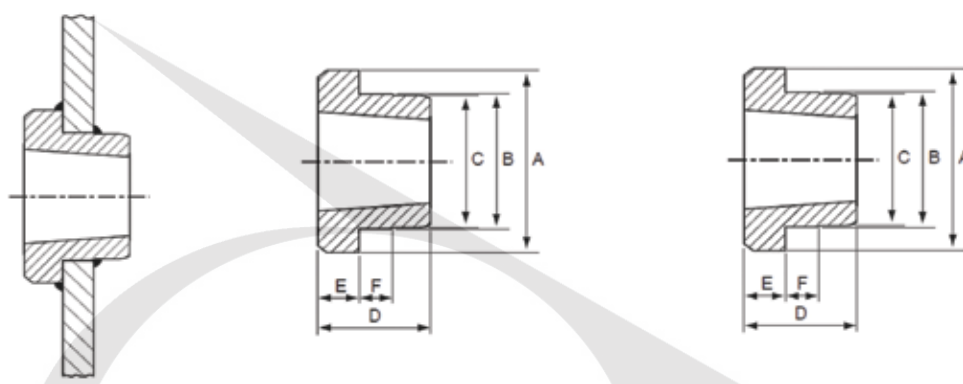
Typical Assembly
