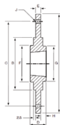
BF Bolt-on-Hub
