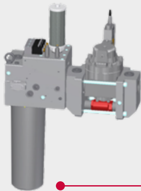
High pressure filter with safety valve ISO 13849 Pld, KAT 3 SF and Dome regulator
