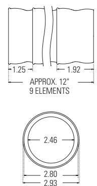
2-1/2" SYSTEM
