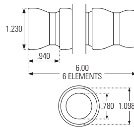
3/4" SYSTEM
