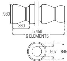
1/2" SYSTEM
