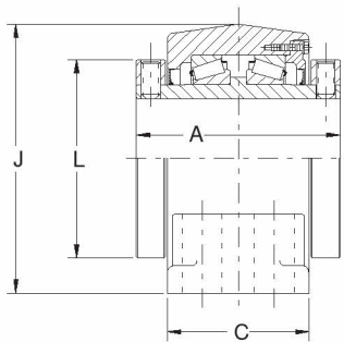
5-7/16" THRU 7" CONSTRUCTION
