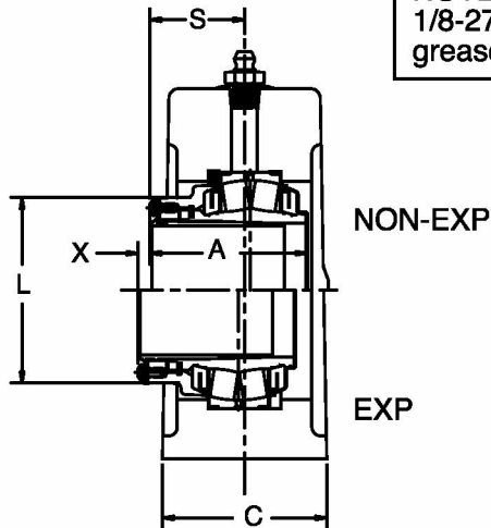
LABYRINTH SEAL
