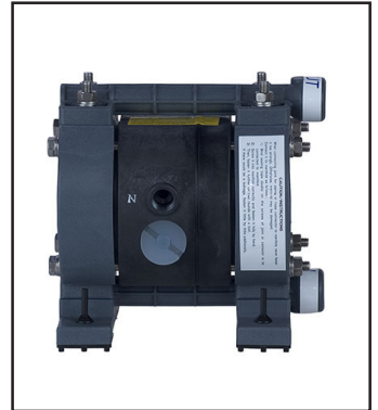
Groundable Acetal Dimensions: 6.14"W x 5.79"H Net Wt.: 3.7 lbs. (1.67 kg) Shipping Wt.: 4.7 lbs.
