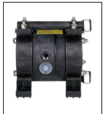
Kynar® Dimensions: 6.14"W x 5.79"H Net Wt.: 3.7 lbs. (1.67 kg) Shipping Wt.: 4.7 lbs.
