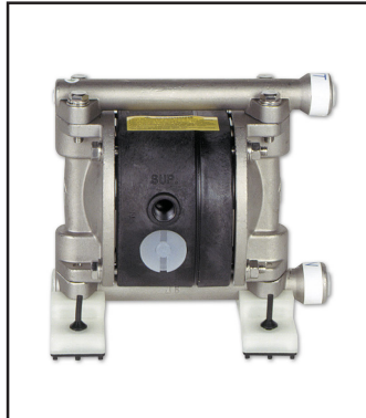
Aluminum Dimensions: 6.1"W x 5.87"H Net Wt.: 3.3 lbs. (1.5 kg) Shipping Wt.: 4.3 lbs.
